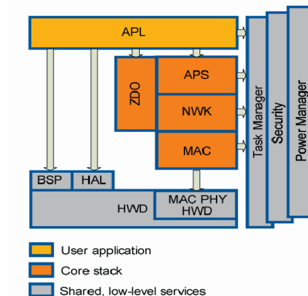
Figure 1. Simplified diagram of the BitCloud software
